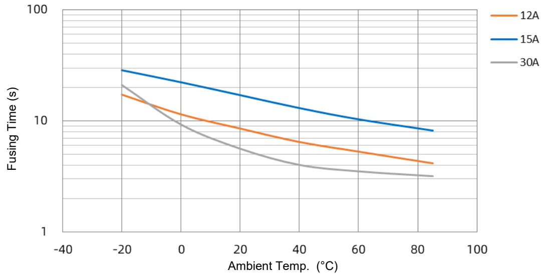
SHL Temp.-Time Curve
