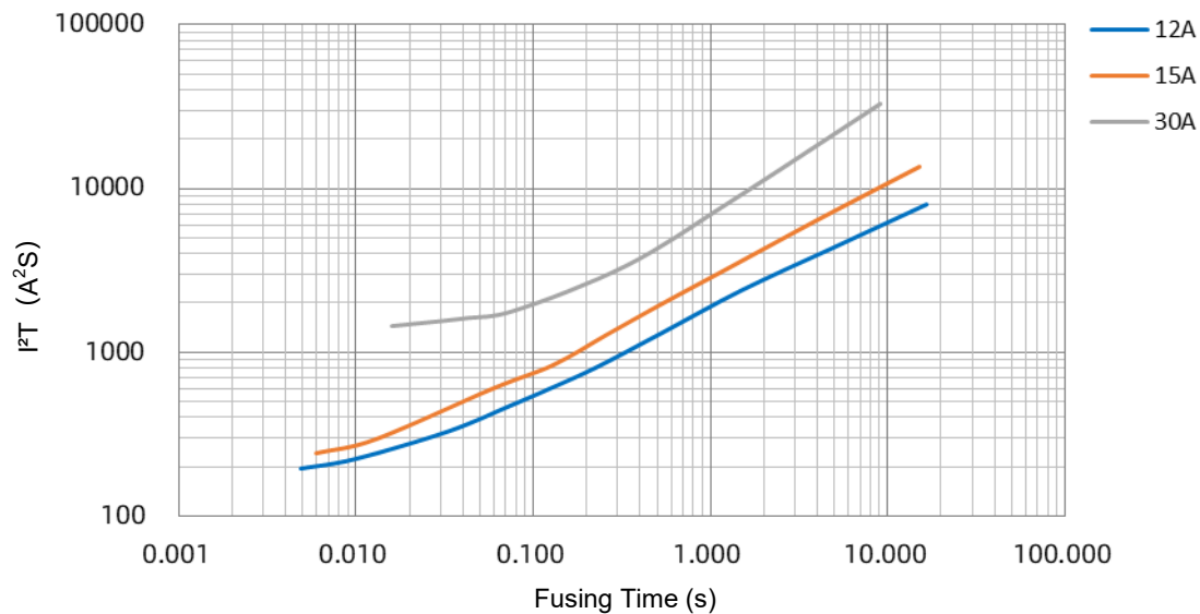
SHL I²t-t Curve
